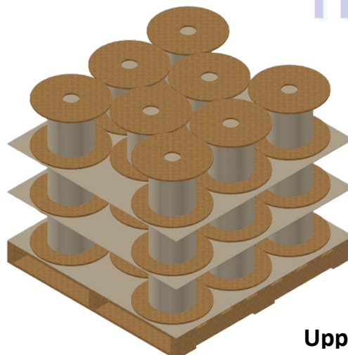
Lower Pallet
